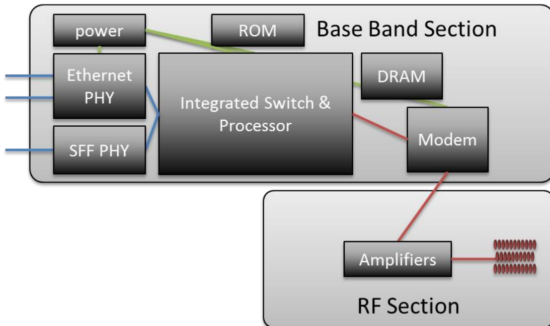
Figure 4: MultiHaul™ B100 Block Diagram
